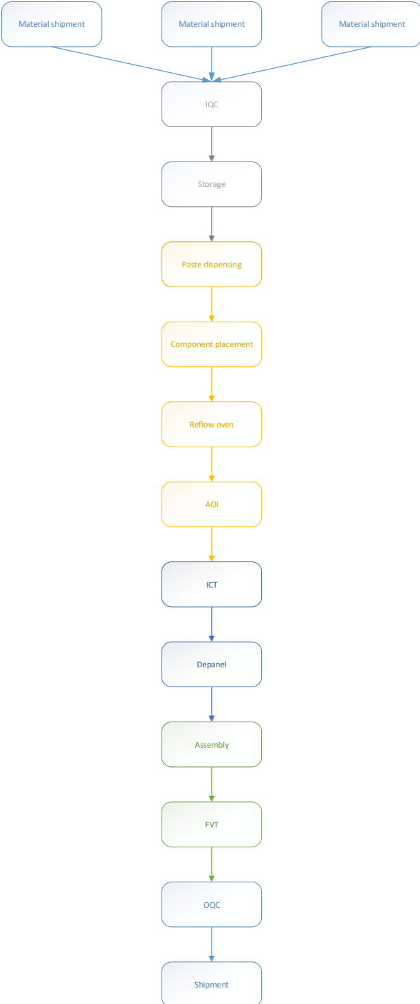
Figure 1: Typical EMS SMT and assembly line (simplified)
